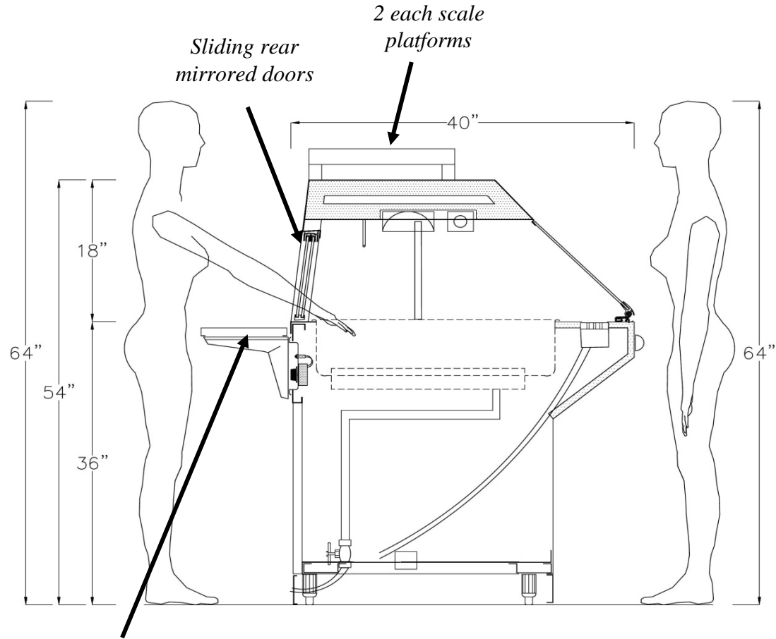
Cross Section
