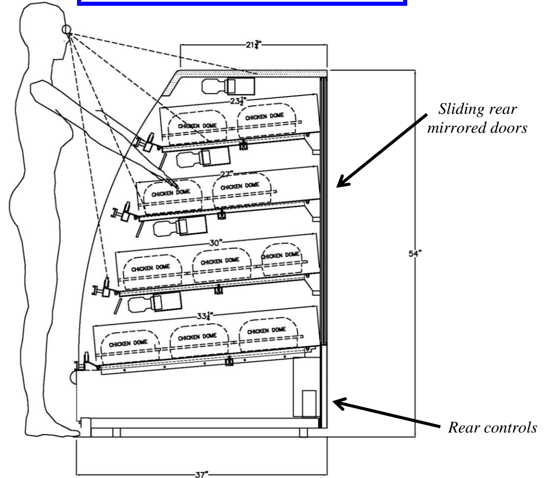
Cross Section
