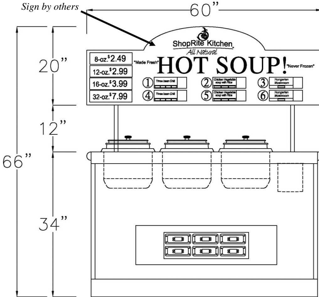
Front Elevation
