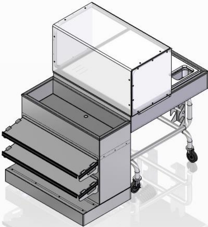
Meat Cutting Kit shown with Half-Canopy Kit and Modular Clam Bar / Dry Shelf Kit
