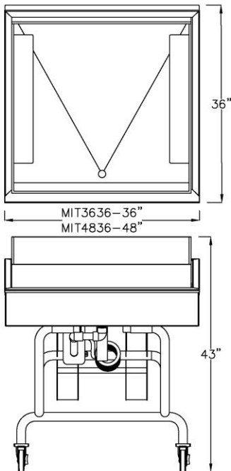
3' MIT3636 shown with Self Service Kit
