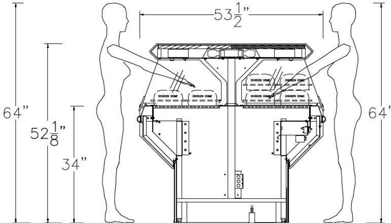
Cross Section
