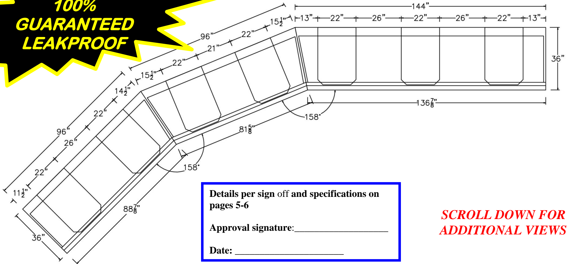
Pedestal plan view
