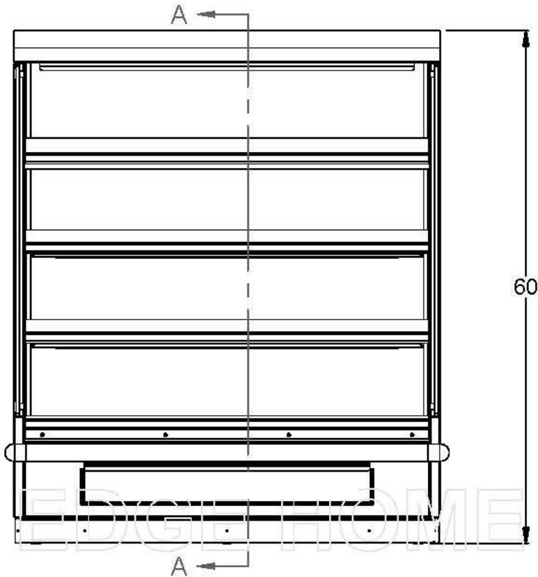
FRONT ELEVATION
