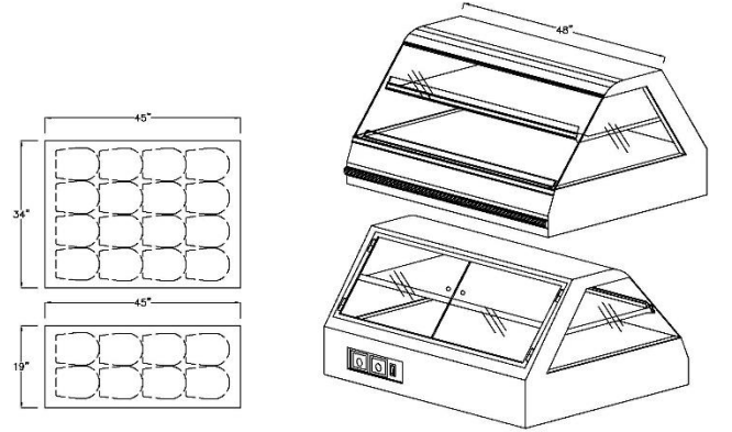
48" CEC2 Two level
