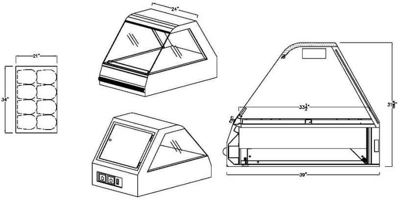
24" CEC One level
