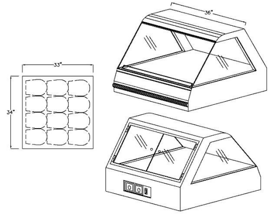
36" CEC One level
