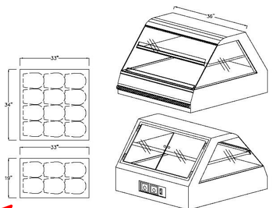
36" CEC2 Two level
