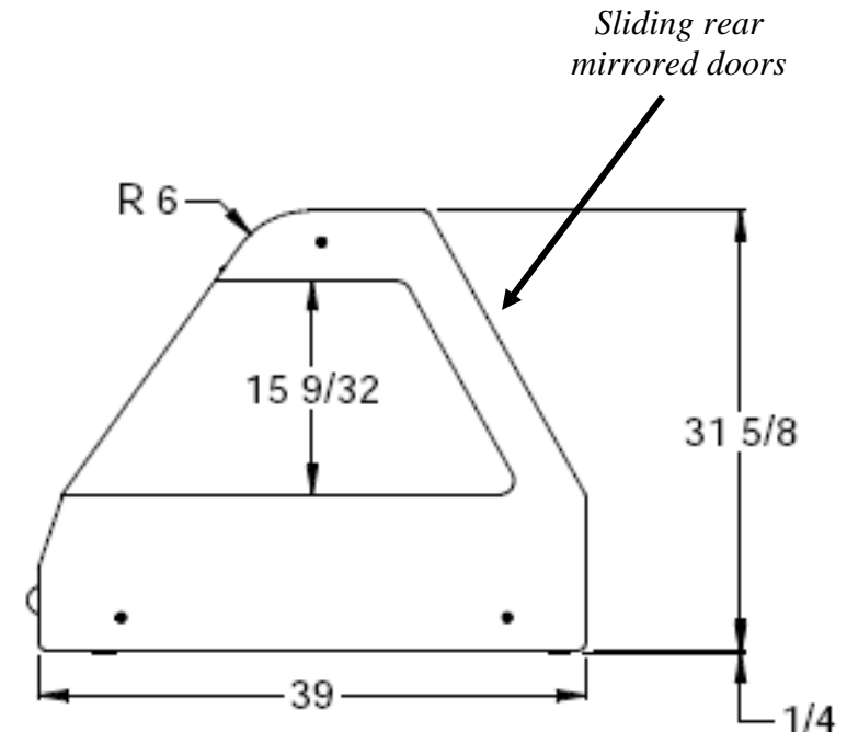
Countertop Model End Section View
