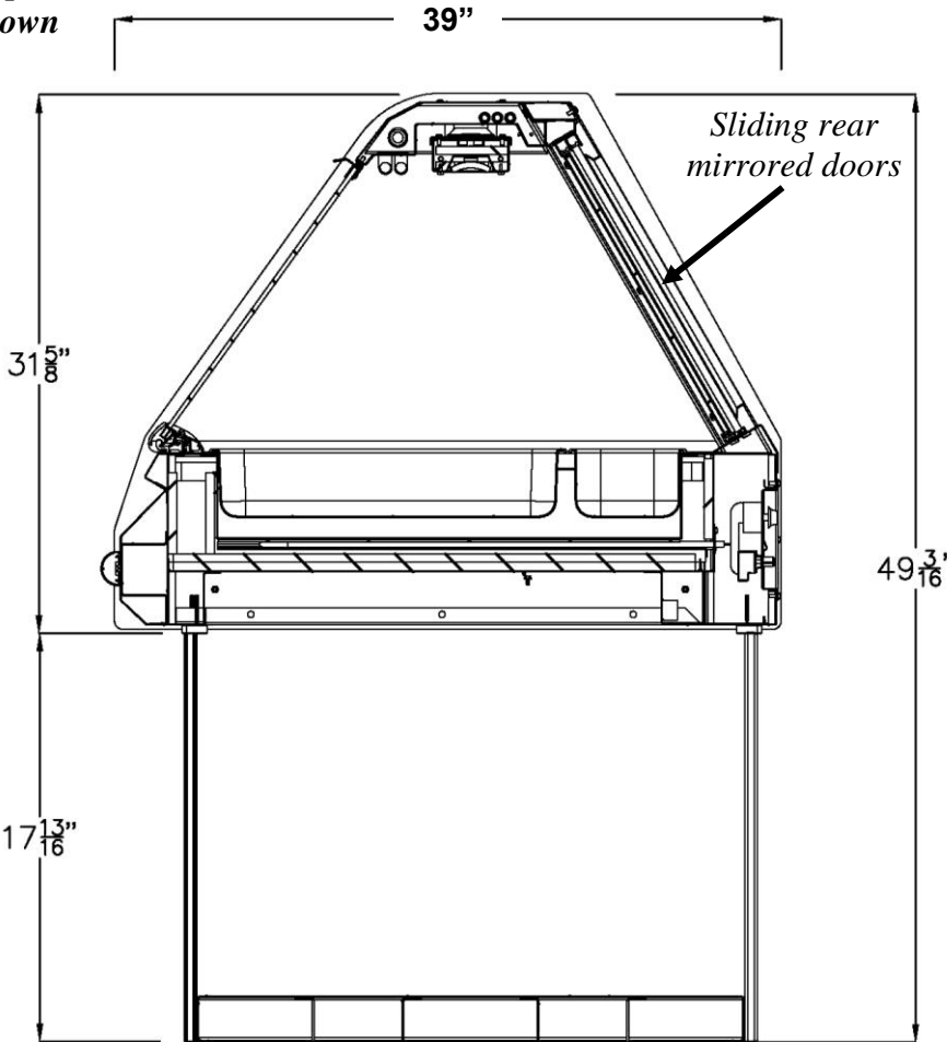
Cross Section
