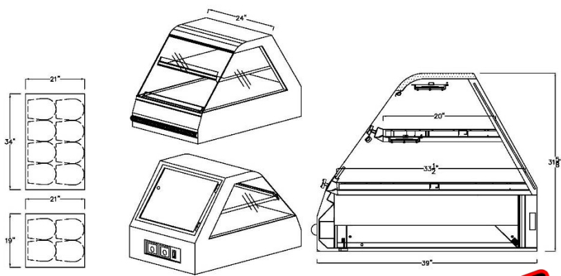
24" CEC2 Two level
