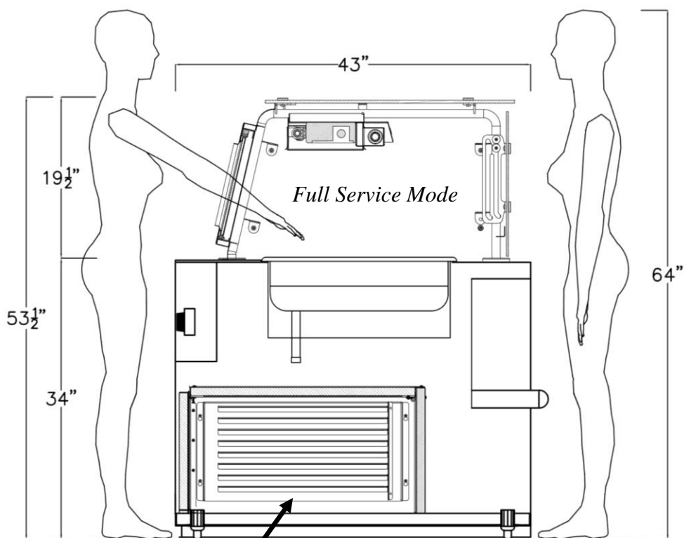
Hot Food Pan Holding Cabinet
